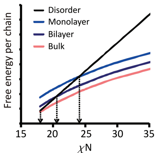
Figure 9. Differences in free energy per chain of the block copolymer in a monolayer, bilayer and bulk phase, compared to the disordered state free energy.
